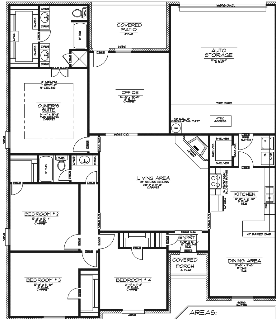
PLAN #38065
